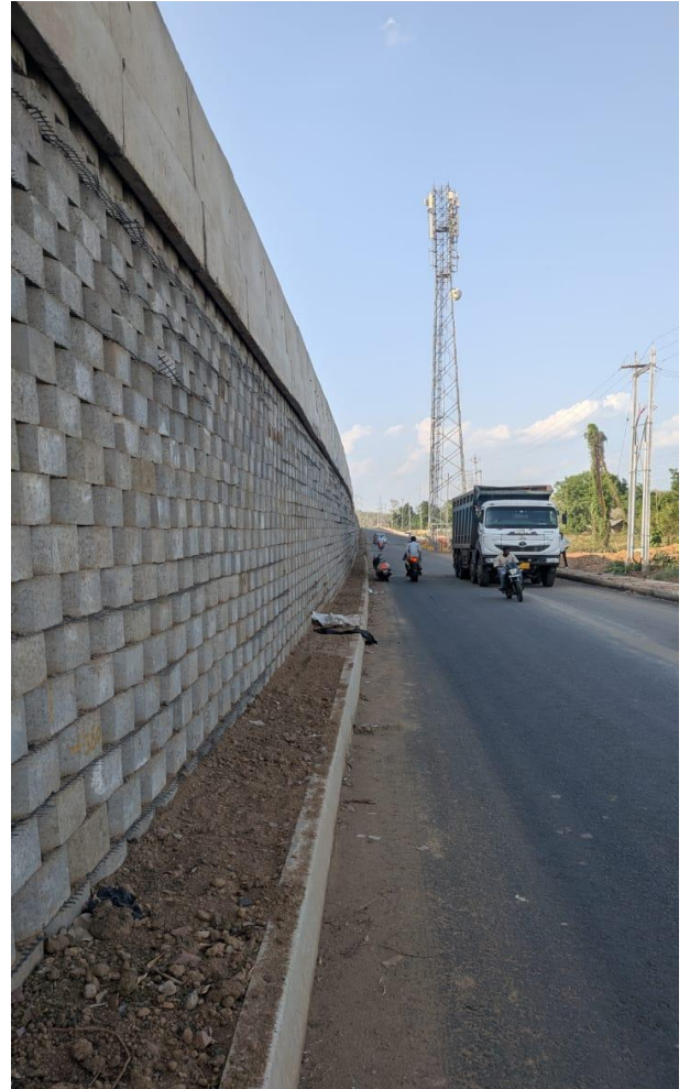
RE Wall work completed @ 92+420
